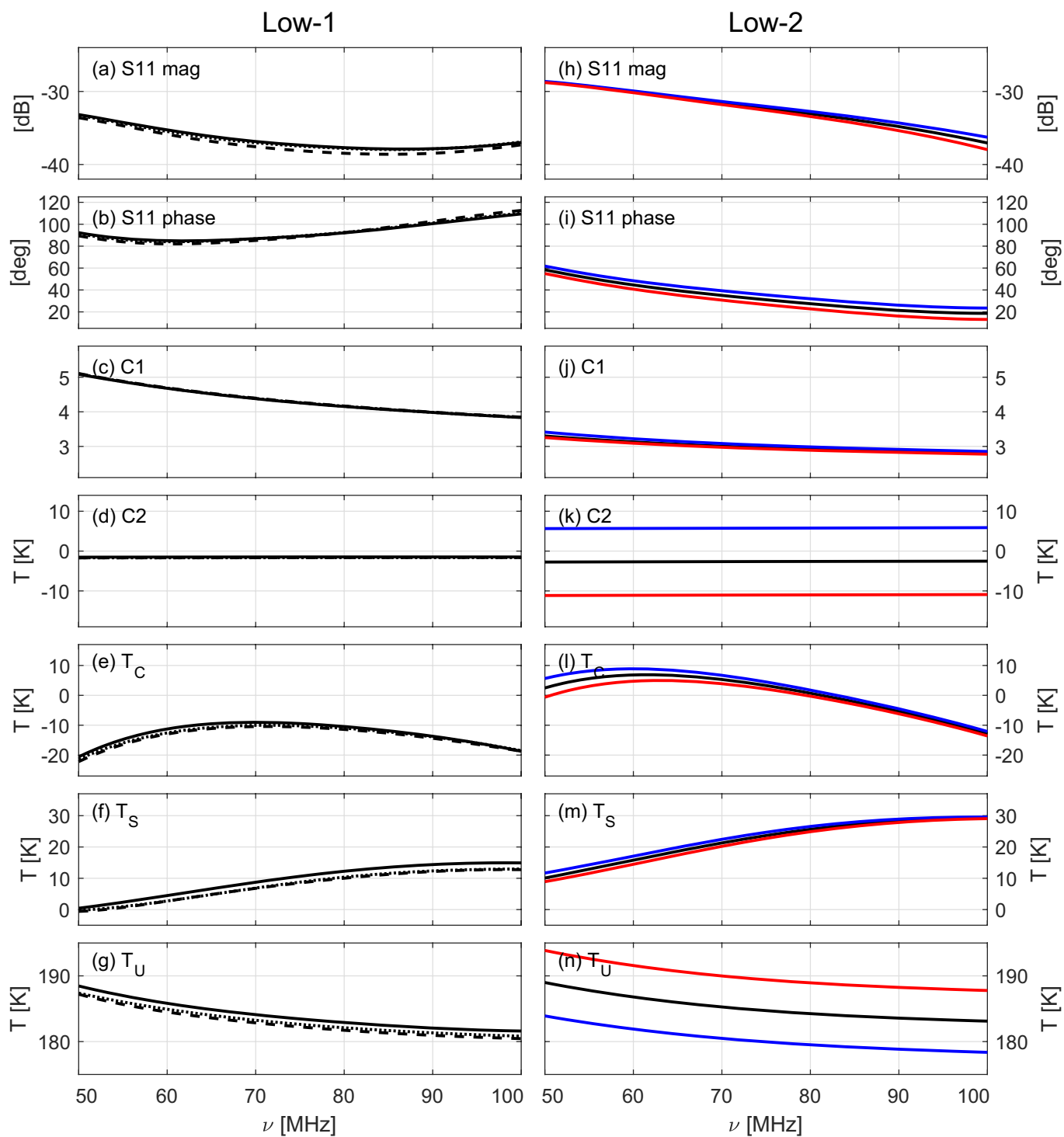
Extended Data Figure 5 | Calibration parameter solutions. a–g, Solutions for the low-1 receiver at its fixed 25 °C operating temperature. It was calibrated on three occasions spanning two years, bracketing all of the low-1 observations reported. The first calibration was in August 2015 before commencing cases H1 and H2 (solid), the next was in May 2017 before H3 (dotted), and the final was in
