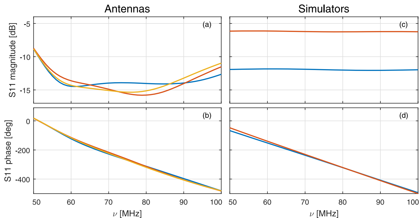
Extended Data Figure 3 | Antenna and simulator reflection coefficients. a, b , Measurements of the reflection coefficient magnitude ( a ) and phase ( b ) are plotted for hardware configurations H2 (blue), H4 (red) and H6 (yellow). The antennas are designed identically (except H6 has the balun shield removed), but are tuned manually during installation by adjusting
