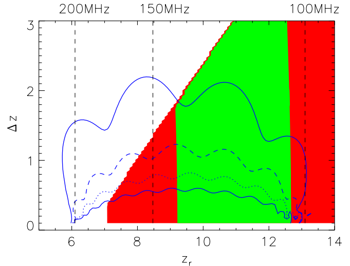
Figure 6. 95% constraint region on a tanh reionization model T_b(z) = T_{21} \tanh[(z - z_r)/\Delta z] of the end of reionization for an EDGES-like experiment assuming N_{\text{poly}} = 3 (solid curve), 6 (dashed curve), 9 (dotted curve) and 12 (dotted-dashed curve). Also plotted are the 68 and 95% contours for the WMAP5 electron scattering optical depth constraint combined with a prior that x_i(z = 6.5) > 0.95 (green and red coloured regions). Reproduced with permission from [97]. Copyright 2010 American Physical Society.
