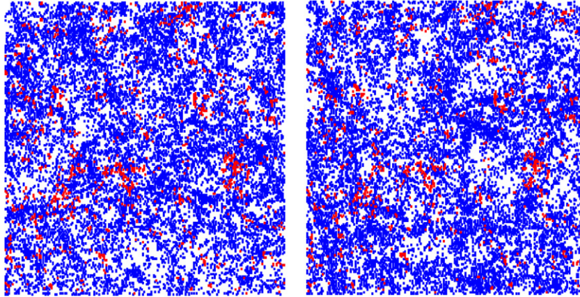
Figure 14. A slice from a simulated realization of line emission from galaxies at an observed wavelength of 441 \mu\text{m} (left) and 364 \mu\text{m} (right) [174]. The slice is in the plane of the sky and spans 250 \times 250 comoving \text{Mpc}^2 with a depth of \Delta\nu/\nu = 0.001 . The colored squares indicate pixels which have line emission greater than 200 \text{ Jy Sr}^{-1} for the left panel and 250 \text{ Jy Sr}^{-1} for the right panel. The emission from O I ( 63 \mu\text{m} ) and O III ( 52 \mu\text{m} ) is shown in red on the left and right panels, respectively, originating from the same galaxies at z = 6 . All of the lines illustrated in figure 13 are included and plotted in blue. Cross-correlating data at these two observed wavelengths would reveal the emission in O I and O III from z = 6 with the other emission lines being essentially uncorrelated. Reproduced with permission from [174]. Copyright 2011 SISSA.
