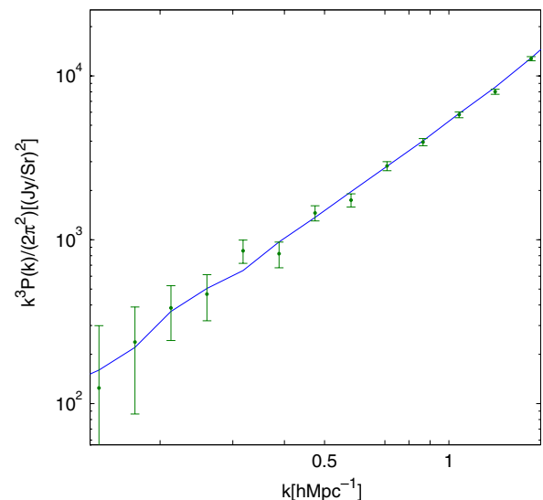
Figure 15. The cross power spectrum of O I ( 63 \mu\text{m} ) and O III ( 52 \mu\text{m} ) at z = 6 measured from mock simulation data for a hypothetical infrared space telescope similar to SPICA [174]. The solid line is the cross power spectrum measured when only line emission from galaxies in the target lines is included. The points are the recovered power spectrum when detector noise, contaminating line emission, galaxy continuum emission and dust in our galaxy and the CMB are included. The error bars follow equation (62) with P_{1\text{total}} and P_{2\text{total}} calculated from the simulated data, including detector noise, contaminating line emission and sample variance. Reproduced with permission from [174]. Copyright 2011 SISSA.
